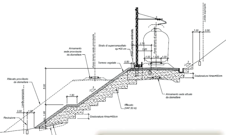
Railway typical cross section
